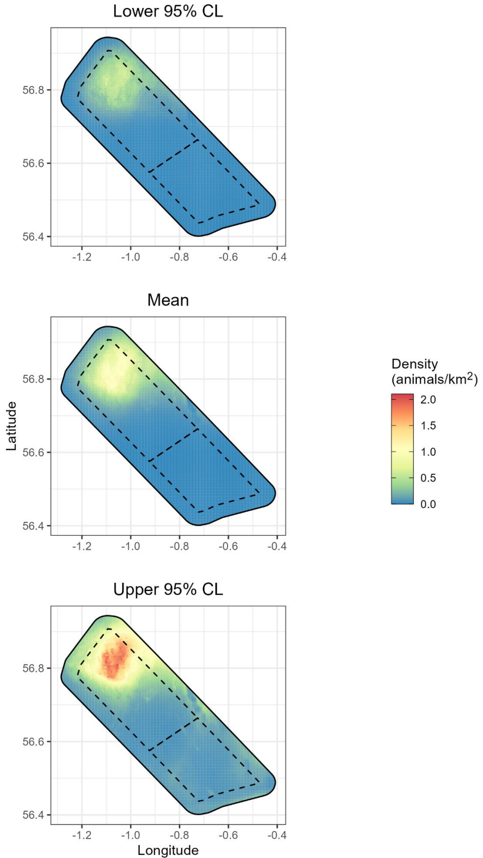
Figure 3.13: Overall predicted mean absolute density of harbour porpoise, with 95% CIs, across the Morven Site Marine Mammal Study Area for the whole 33 month period of digital aerial survey data. Dashed line indicates the Morven North and Morven South Boundaries
