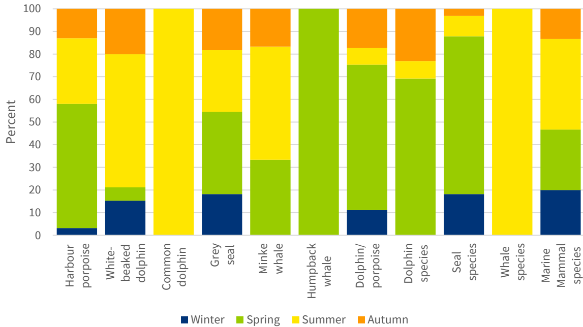
Figure 3.1: Seasonal percentage of marine mammal sightings in the Morven Site Marine Mammal Study Area (P)
