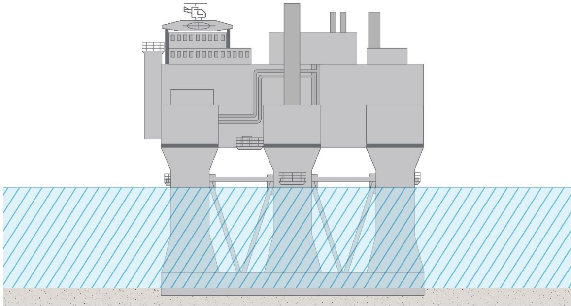
Figure 4.9: Schematic of a typical rectangular gravity base foundation with six legs (not to scale)
